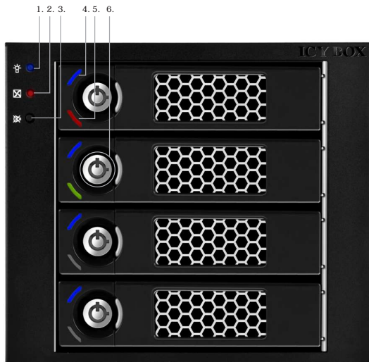
Front view IB-554SSK
