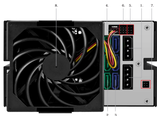
Rear view IB-553SSK
