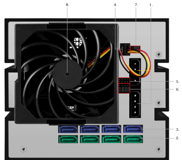
Rear view IB-554SSK
